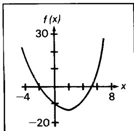
Graph of f(x)
