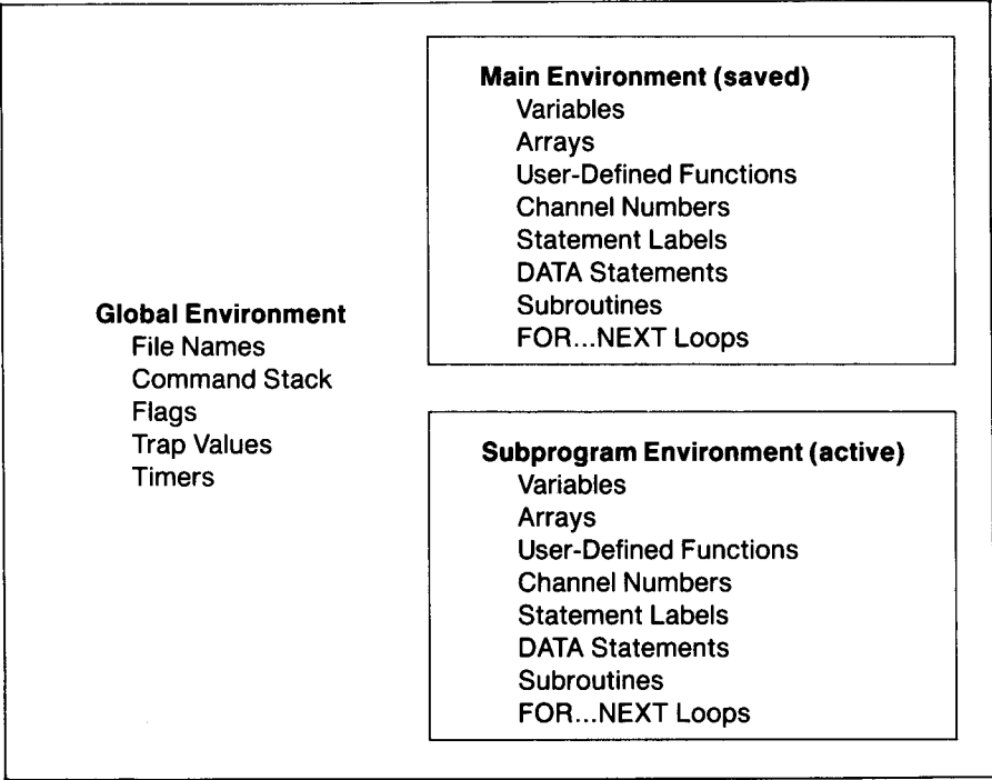
Global, Main, and Subprogram Environments
