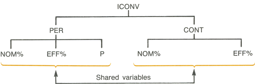
Figure 4-14. Shared Variables
