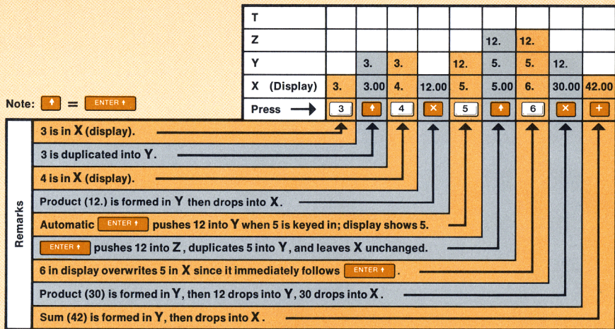
Figure 4. Stack Operations
