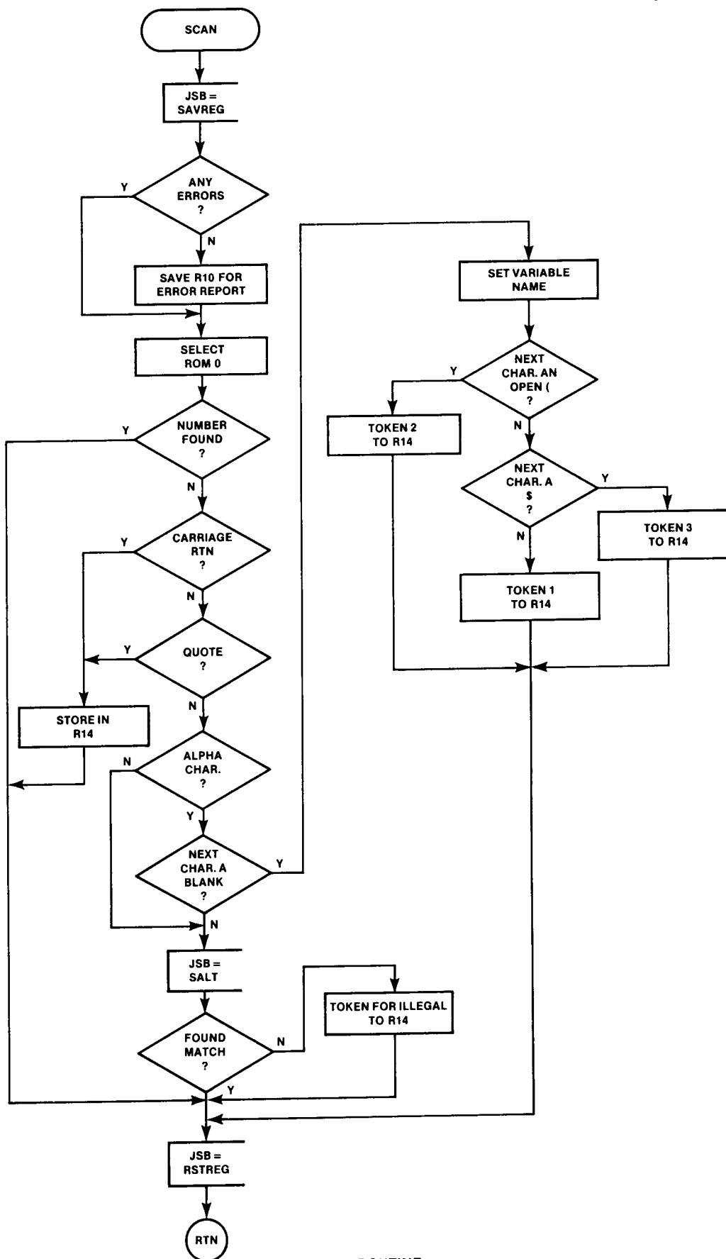
SCAN ROUTINE
