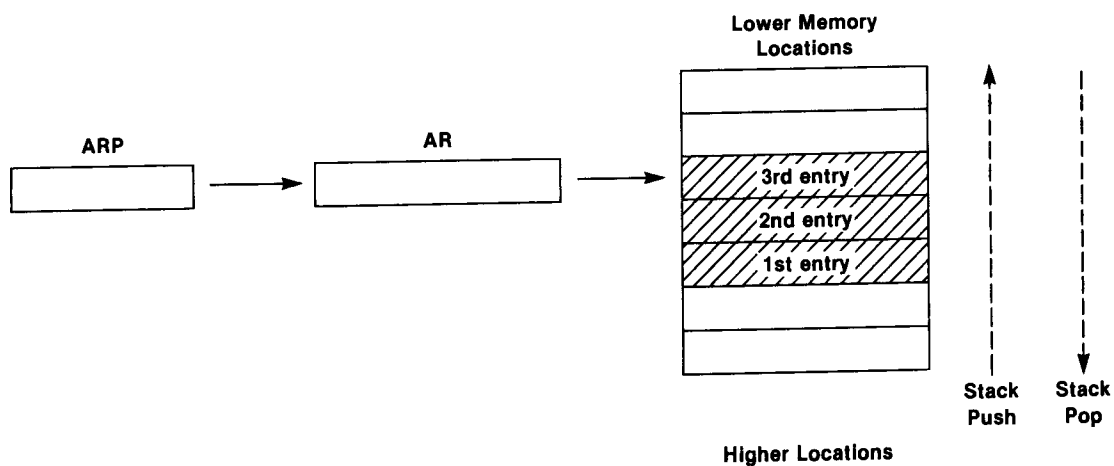
DECREASING STACK
