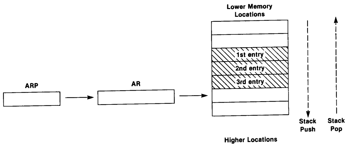
INCREASING STACK
