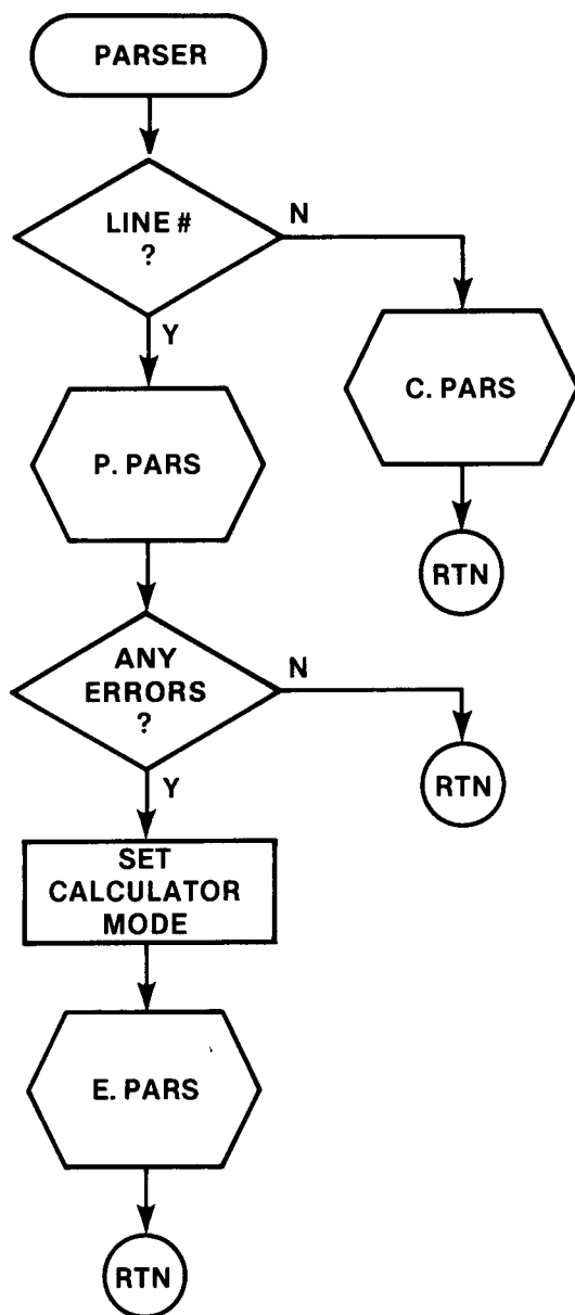
MAIN PARSE LOOP
