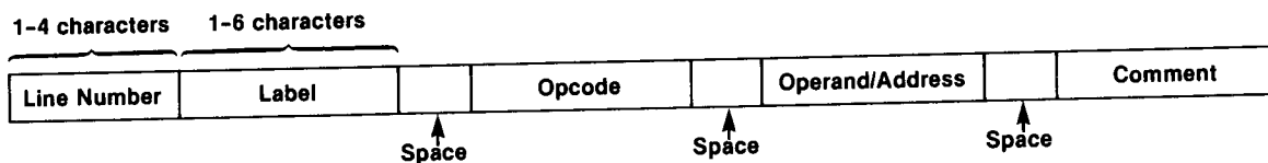
SOURCE CODE INSTRUCTION FORMAT
