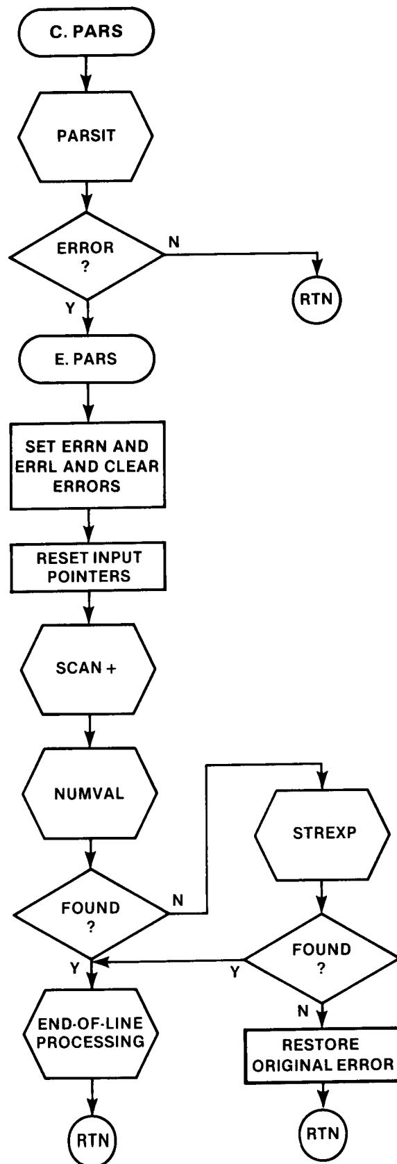
PARSING A CALCULATOR MODE STATEMENT
