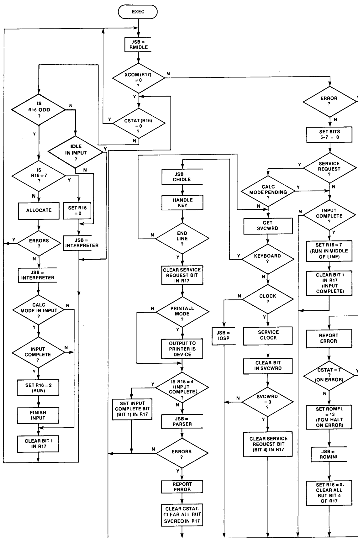
EXECUTIVE LOOP
