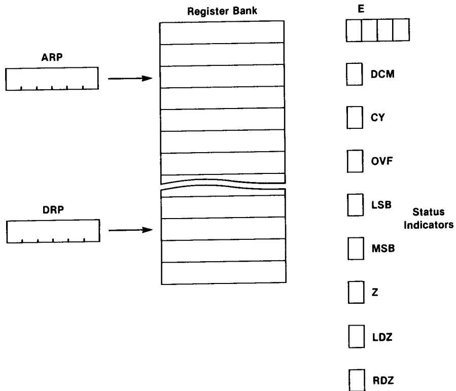
CENTRAL PROCESSING UNIT
