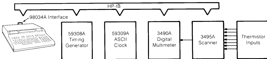
A Typical HP-IB System
