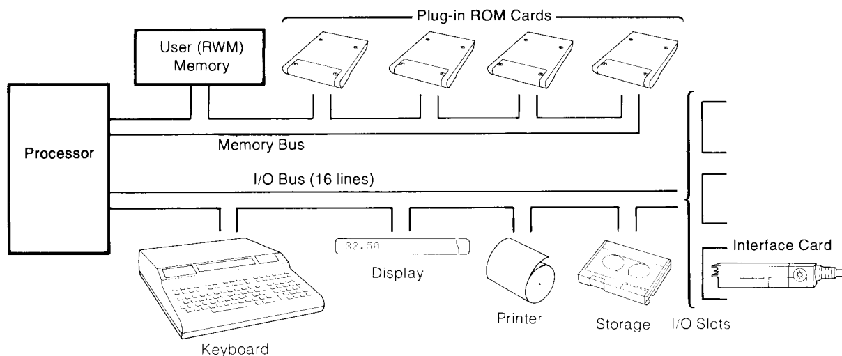
The Calculator Input/Output Scheme
