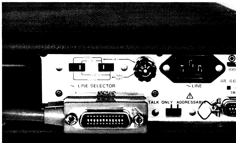
Connecting Bus Cables
