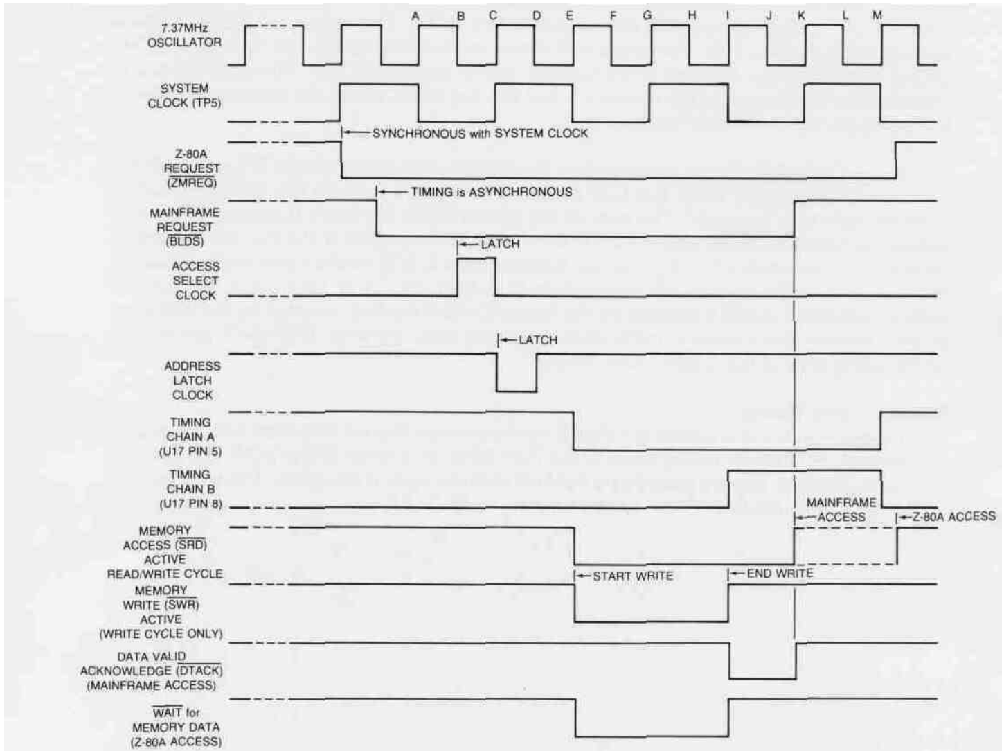
Memory Cycle Timing Diagram
