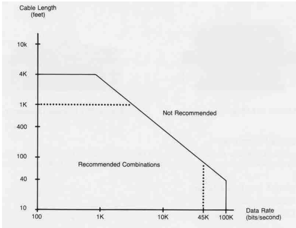
RS-423 Modulation Rate Versus Cable Length
