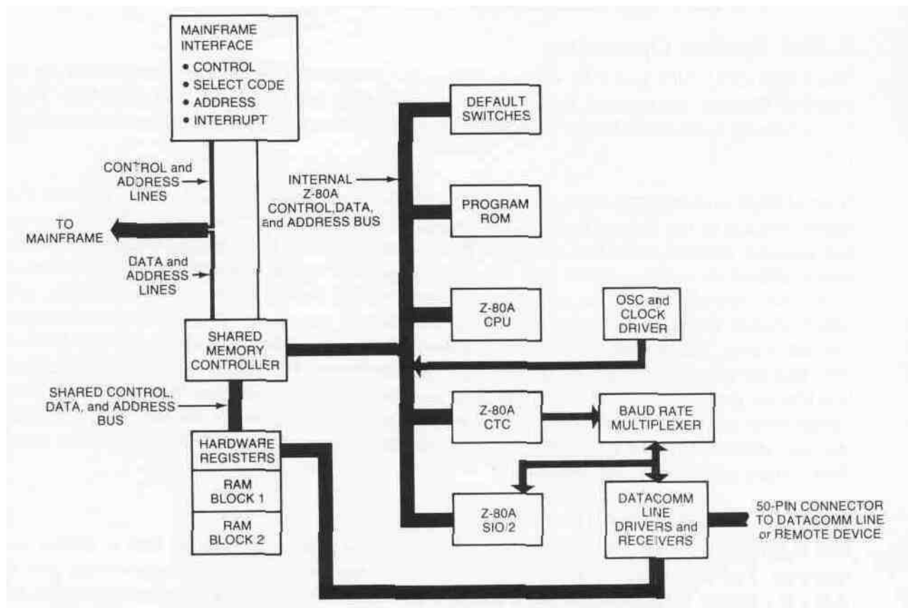
Datacomm Interface Block Diagram
