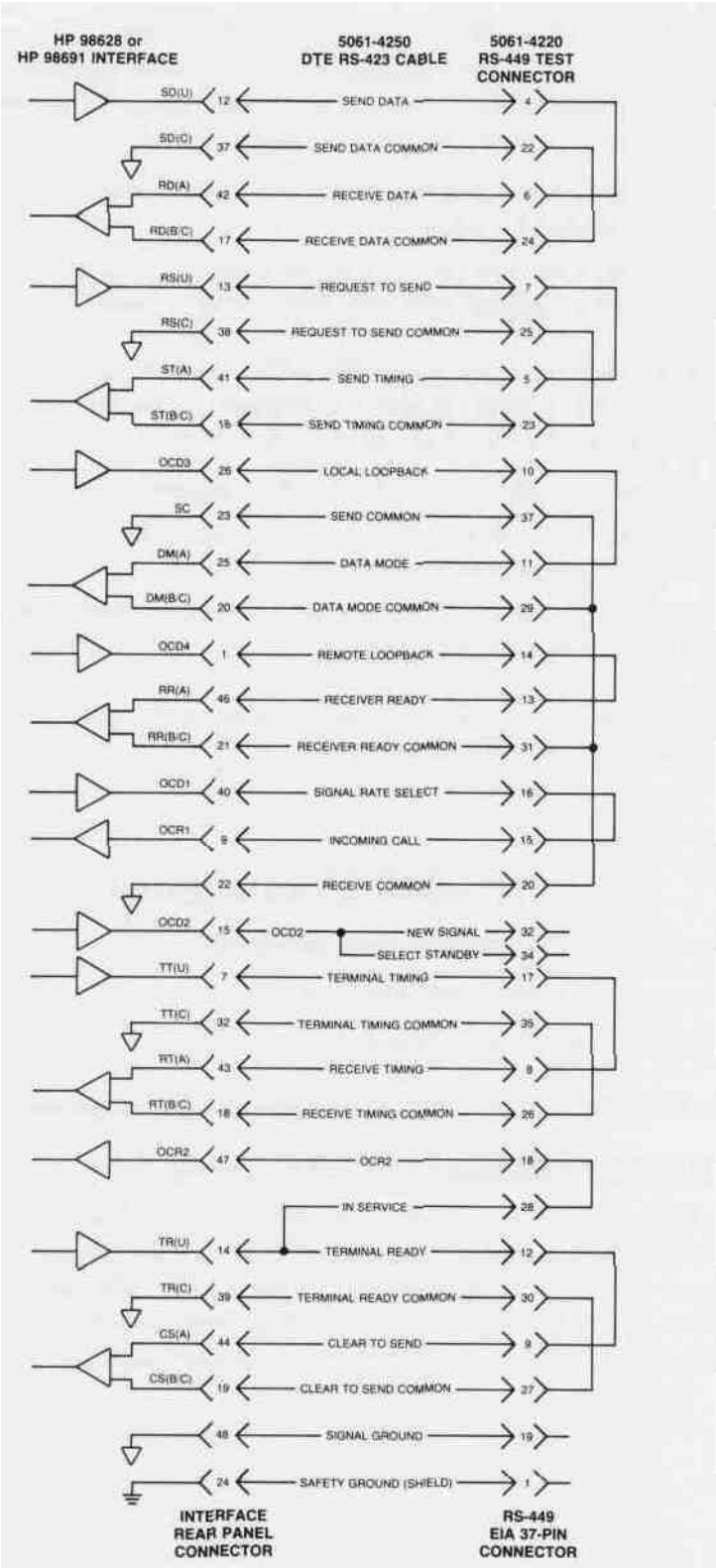
RS-423 Unbalanced-line Interface Cable
