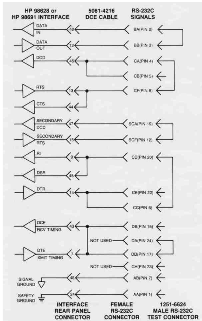
Option 002 DCE Interface Cable and Test Connector
