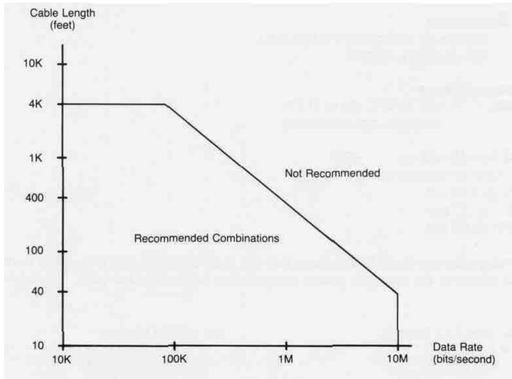
RS-422 Modulation Rate Versus Cable Length
