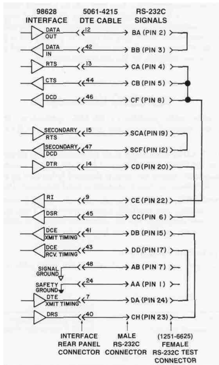
Option 001 DTE Interface Cable and Test Connector
