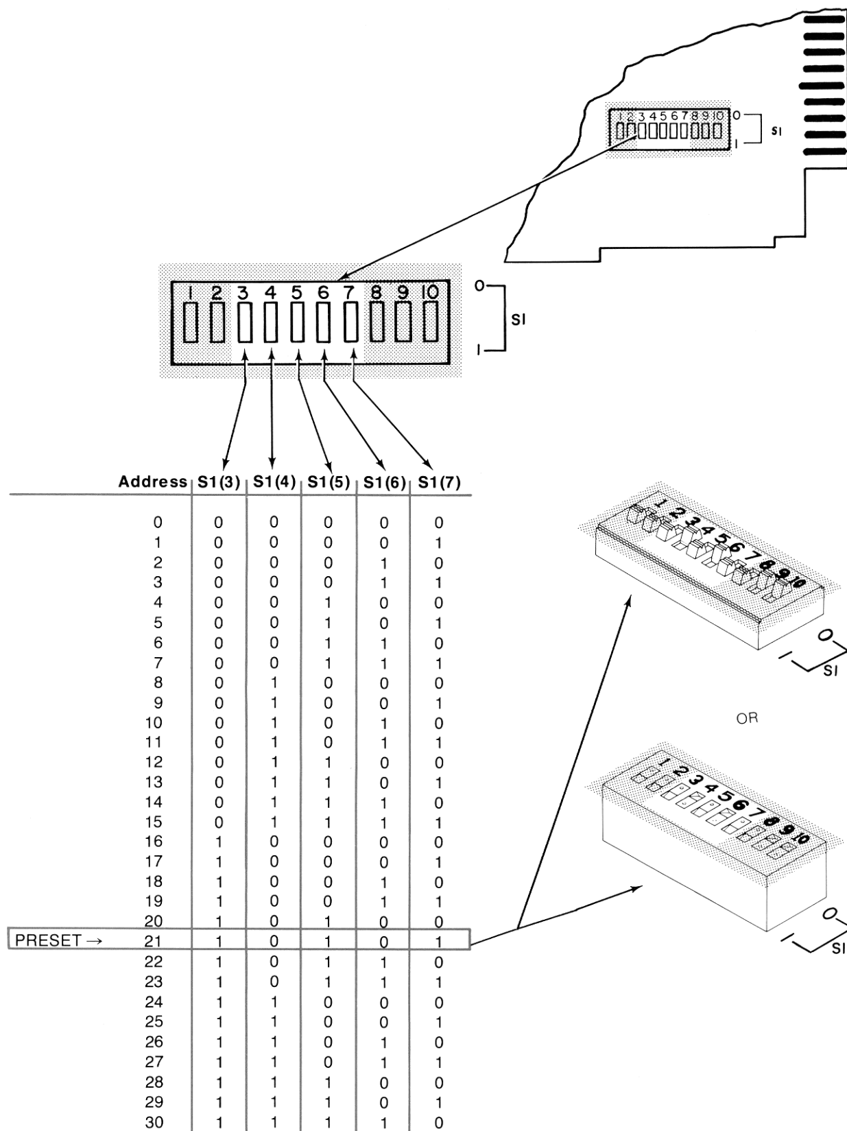
Figure 2-3. Talk/Listen Address Switches
