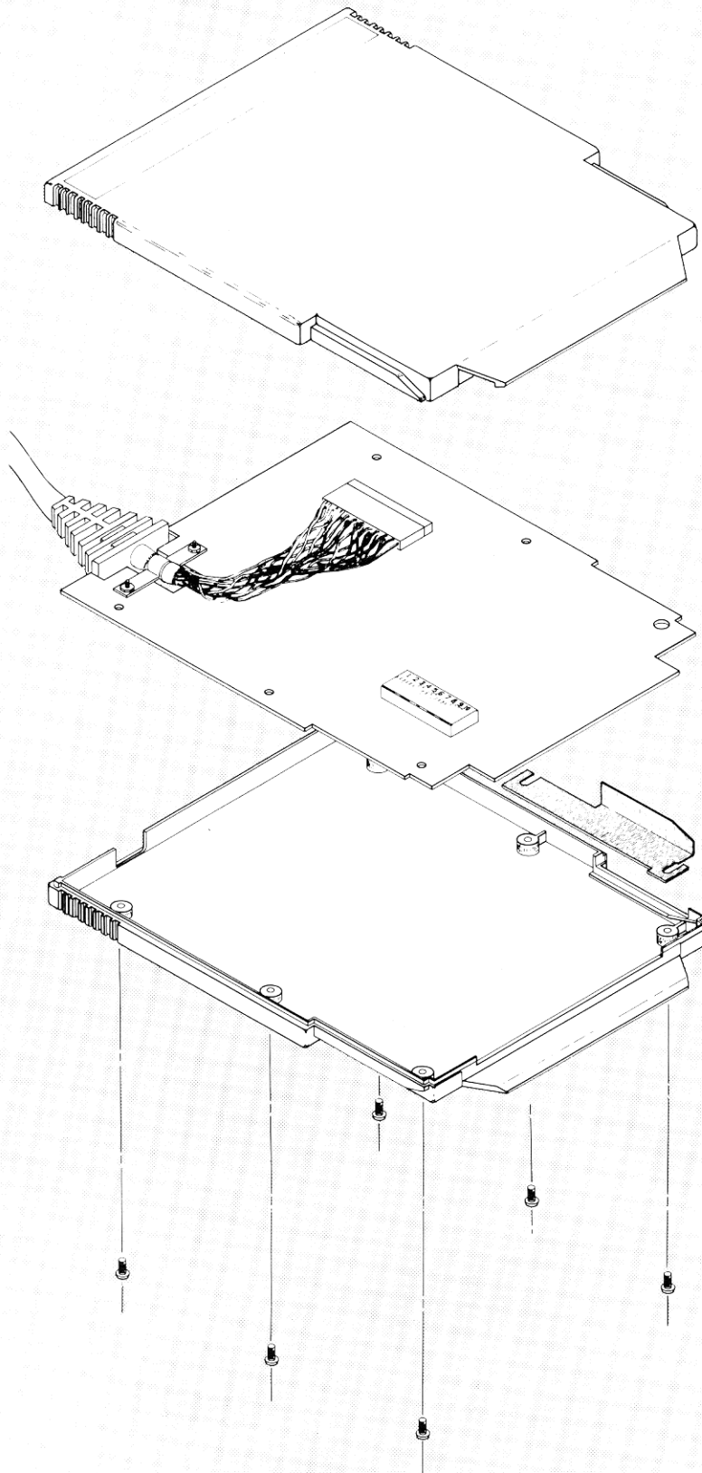
Figure 2-1. Disassembly
