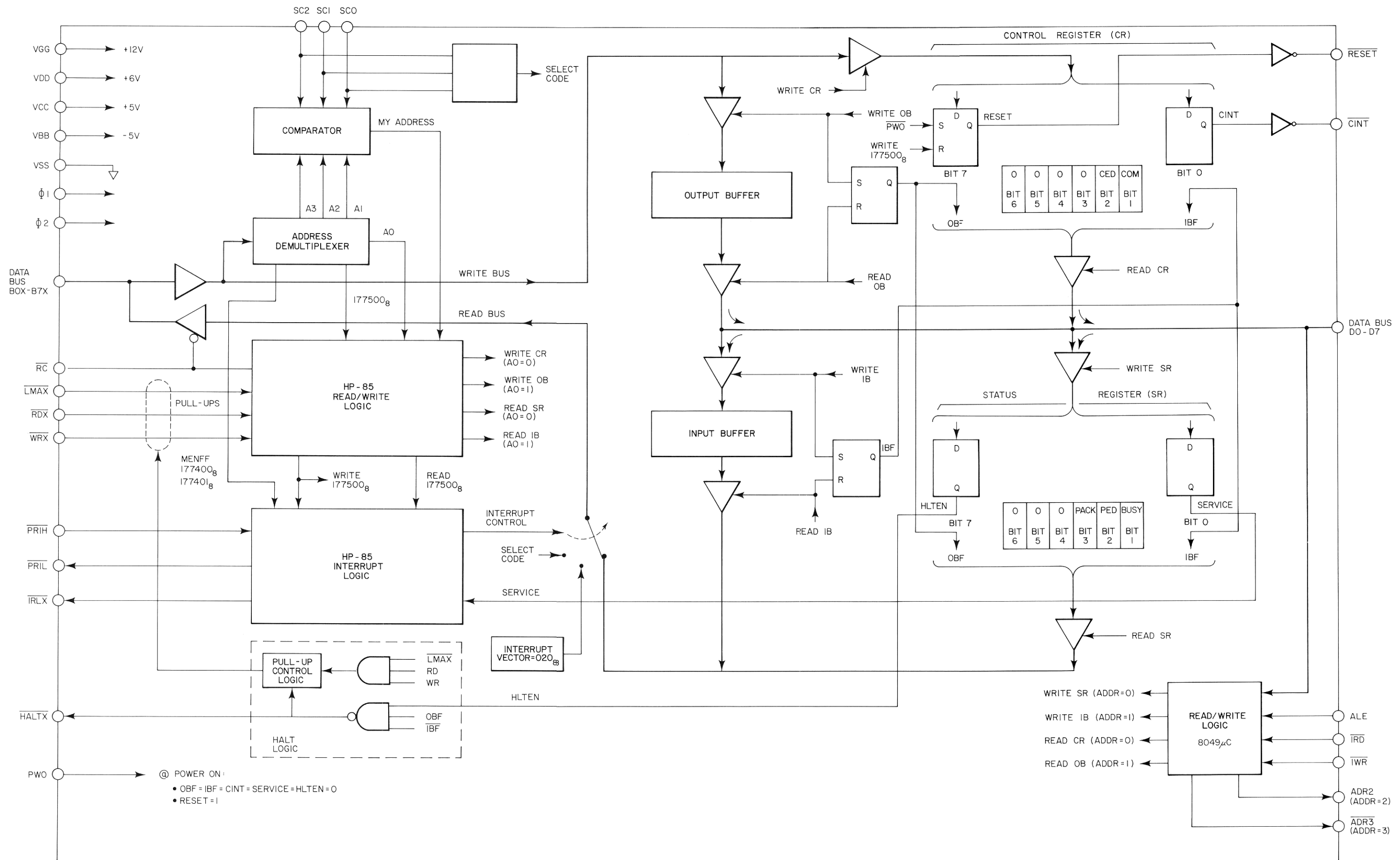
Figure 3-1. Translator IC Block Diagram
