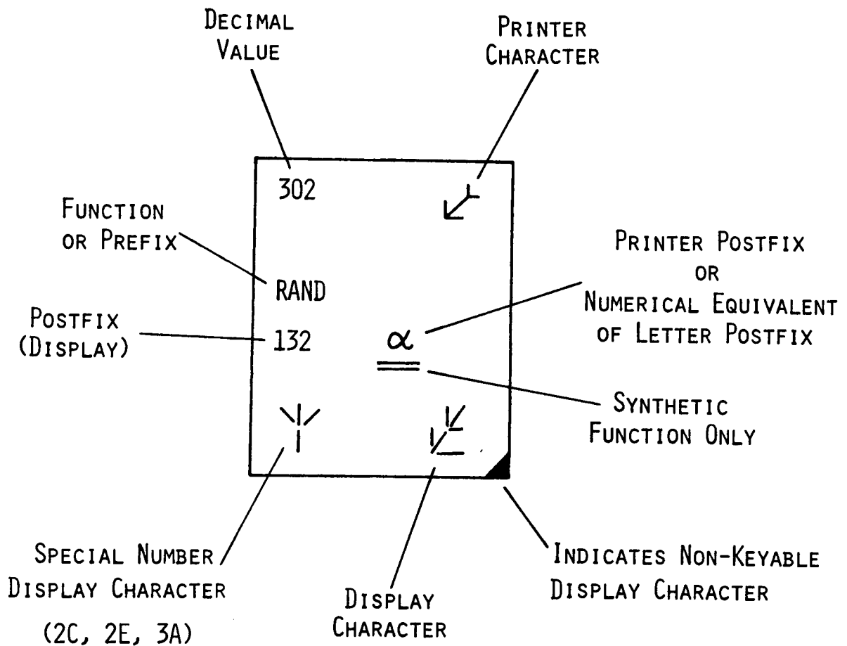
FIGURE 2-4. SAMPLE BYTE TABLE "Box"
