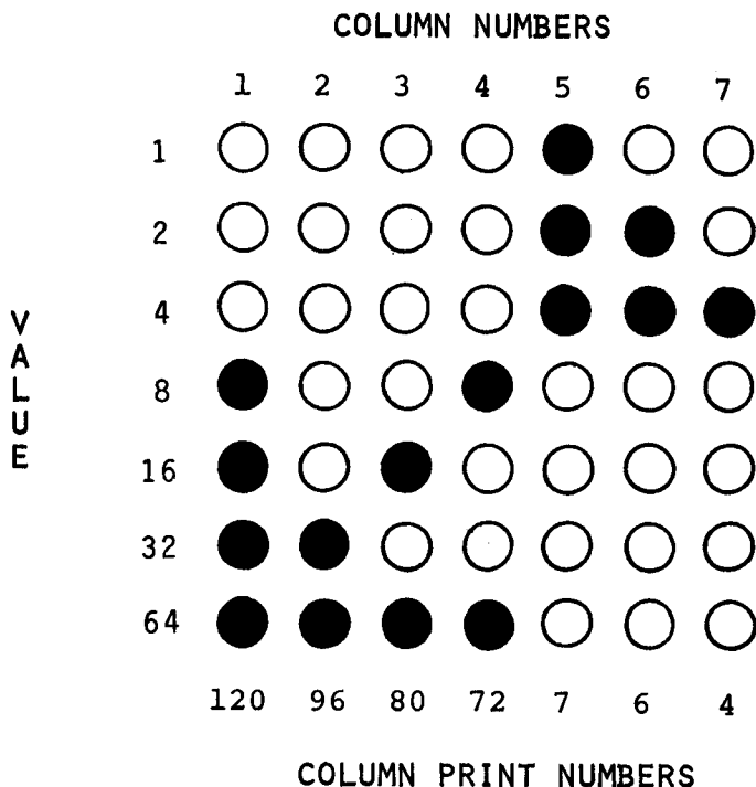
FIGURE 6-1. A SPECIAL GRAPHICS CHARACTER
