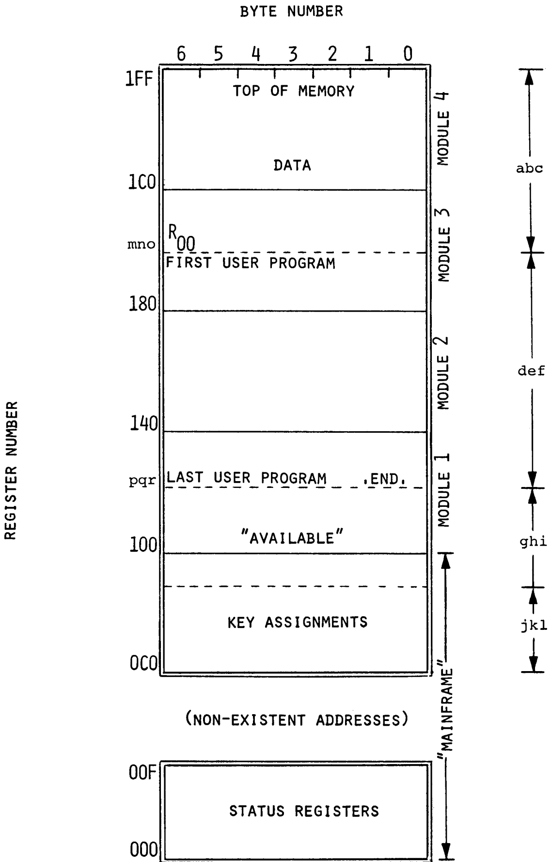
FIGURE 2-5. HP-41C User Memory Partioning
