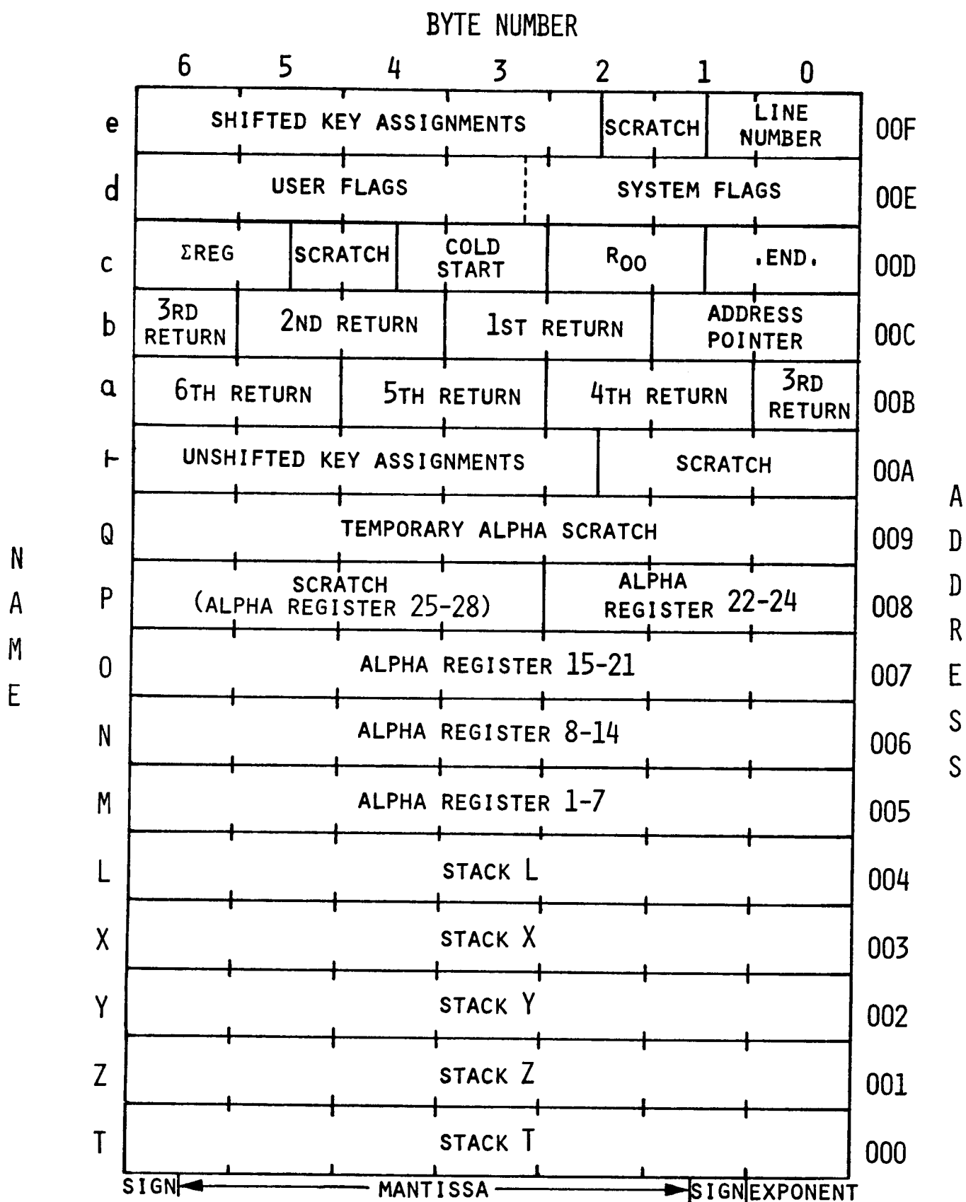
FIGURE 4-1. THE STATUS REGISTERS
