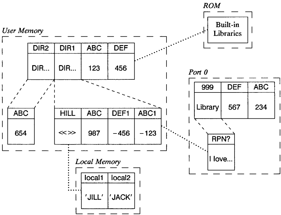
Figure 5.2. Example Memory Organization
