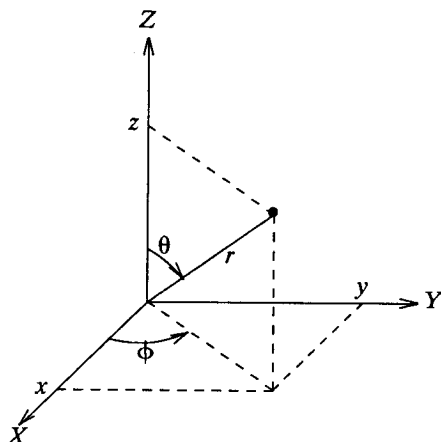
Spherical Polar Coordinates
