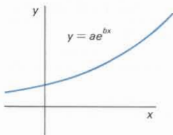
Exponentielle Regression Code = 1
