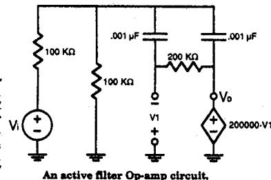
An active filter Op-amp circuit.
