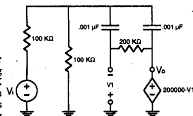
An active filter Op-amp circuit.
