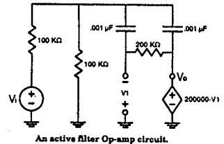
An active filter Op-amp circuit.
