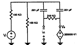
An active filter Op-amp circuit.
