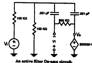
An active filter Op-amp circuit.
