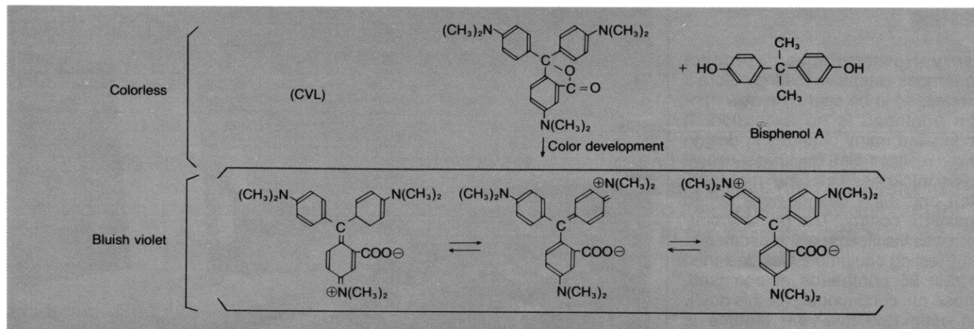
Figure 2. Typical thermal paper chemical reaction.
