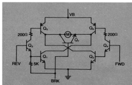
Figure 3. Transistor bridge circuit that forms the basic structure of the motor driver.
