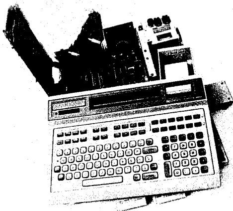
Fig. 1. 9825A Calculator is fully operational when opened for servicing. Printed circuit boards are hinged to provide access to both sides. Plug-in ROMs at front and side were pulled halfway out for this photo.
