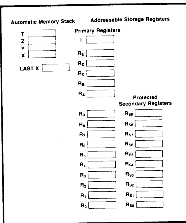
Fig. 4. The HP-67 and HP-97 have a four-register operational stack and a register that retains the last number in the X-register, which is the display register. There are 26 addressable data storage registers, including the I-register, that can be used for indirect control. Protected secondary registers cannot be accessed directly with STO and RCL keys. These registers are used most often for statistical functions and programming, but they can be accessed from the keyboard using the P \Rightarrow S key.
