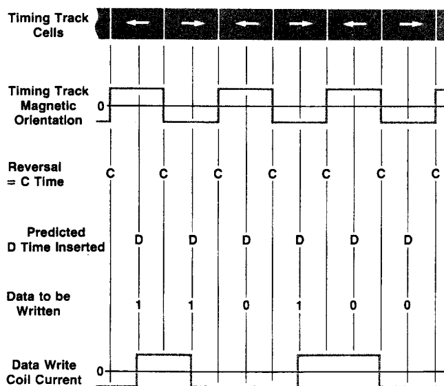
Fig. 7. Write operation timing for HP-75 card recorder.
