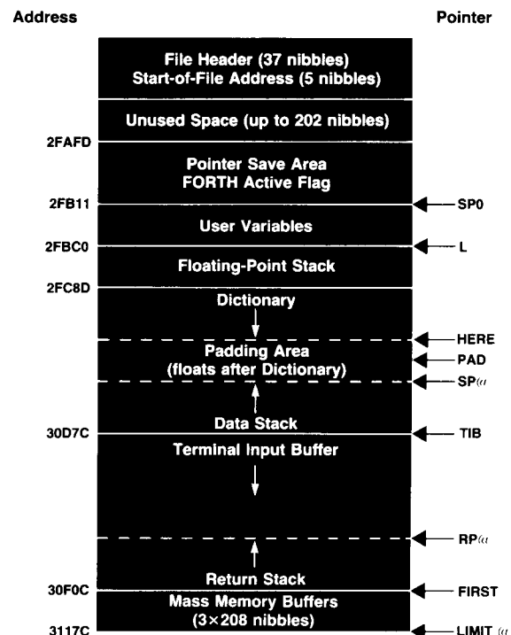
Fig. 1. Structure of the FORTHAM file in the HP-71B's file chain.
