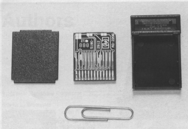
Fig. 2. Exploded view of a typical plug-in module for the HP-71B. The ROM is surface-mounted on the underside of the printed circuit board in the center.
