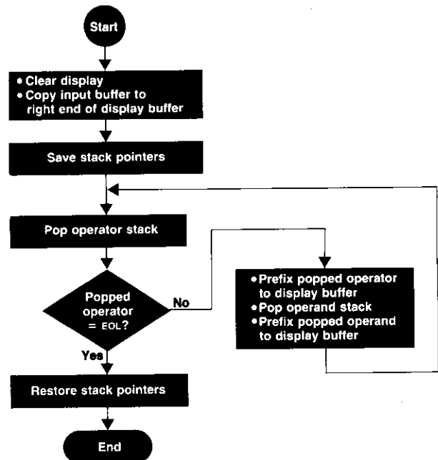
Fig. 2. Decompiler flowchart.
