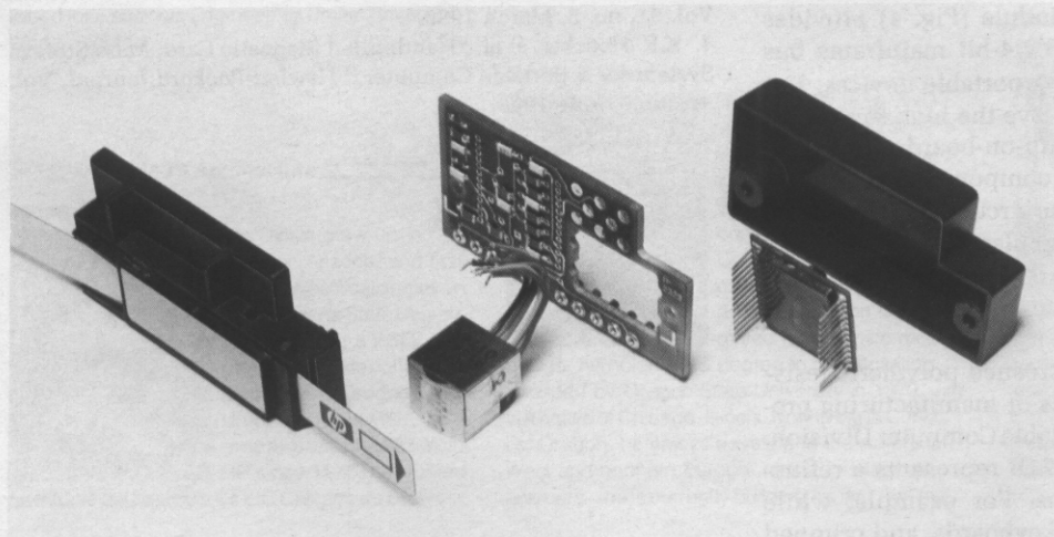
Fig. 3. Exploded view of the optional 82400A Card Reader Module for the HP-71B.
