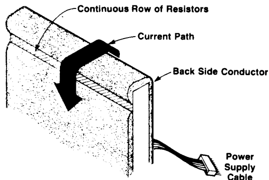
Fig. 3. Current path in the System 45 printhead is from the back of the printhead over the edge.
