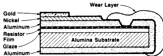
Fig. 4. Cross-section of the thin-film System 45 printhead.
