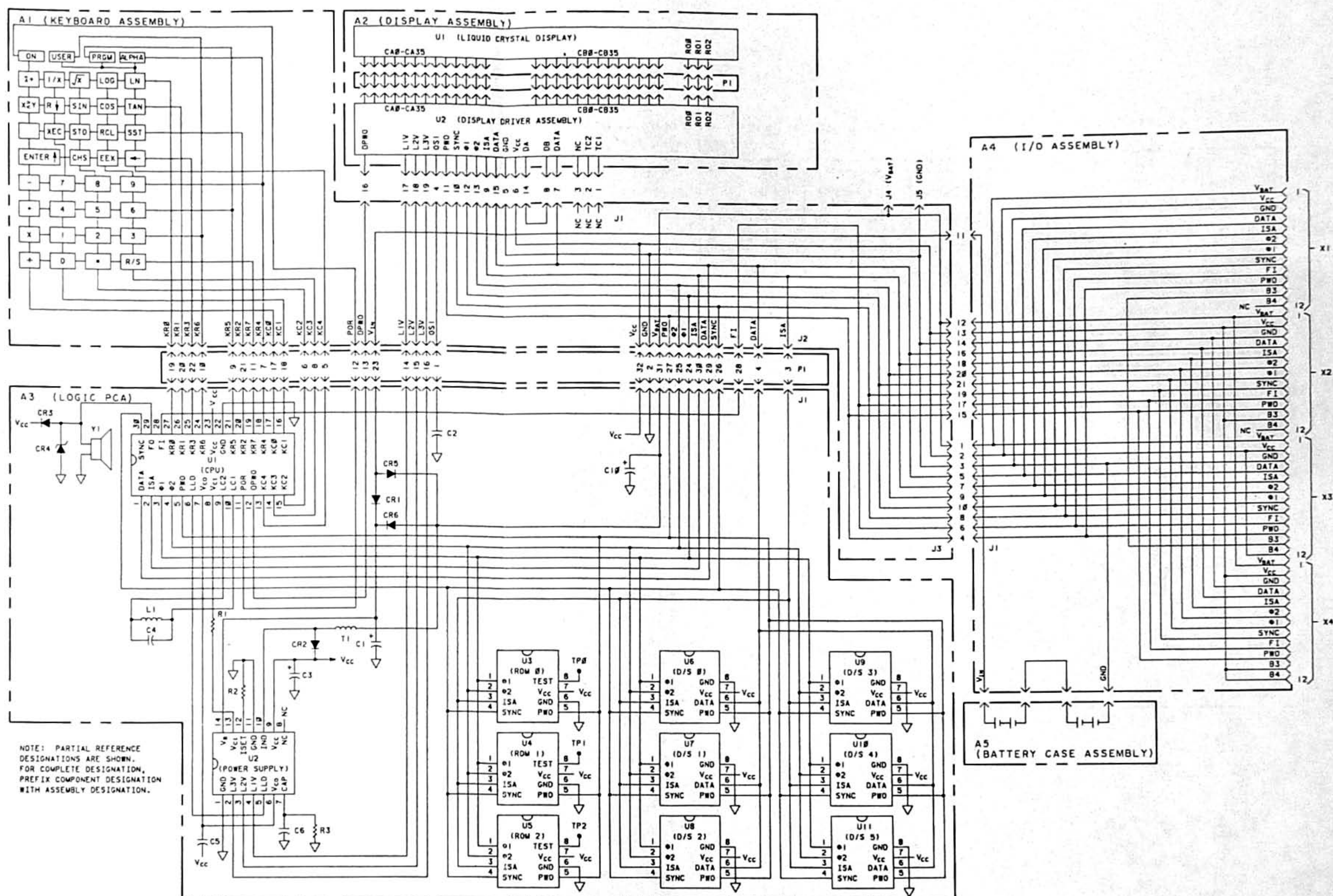
Figure 4-9e. HP-41C/CV Common Board Schematic Diagram
