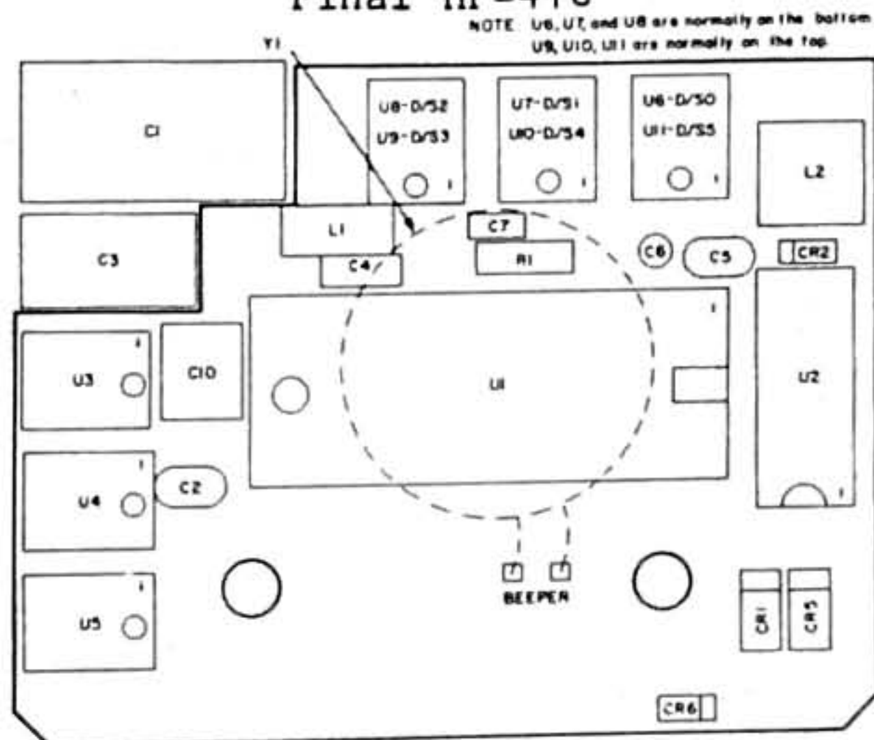
HP-41C/CV Common Board
