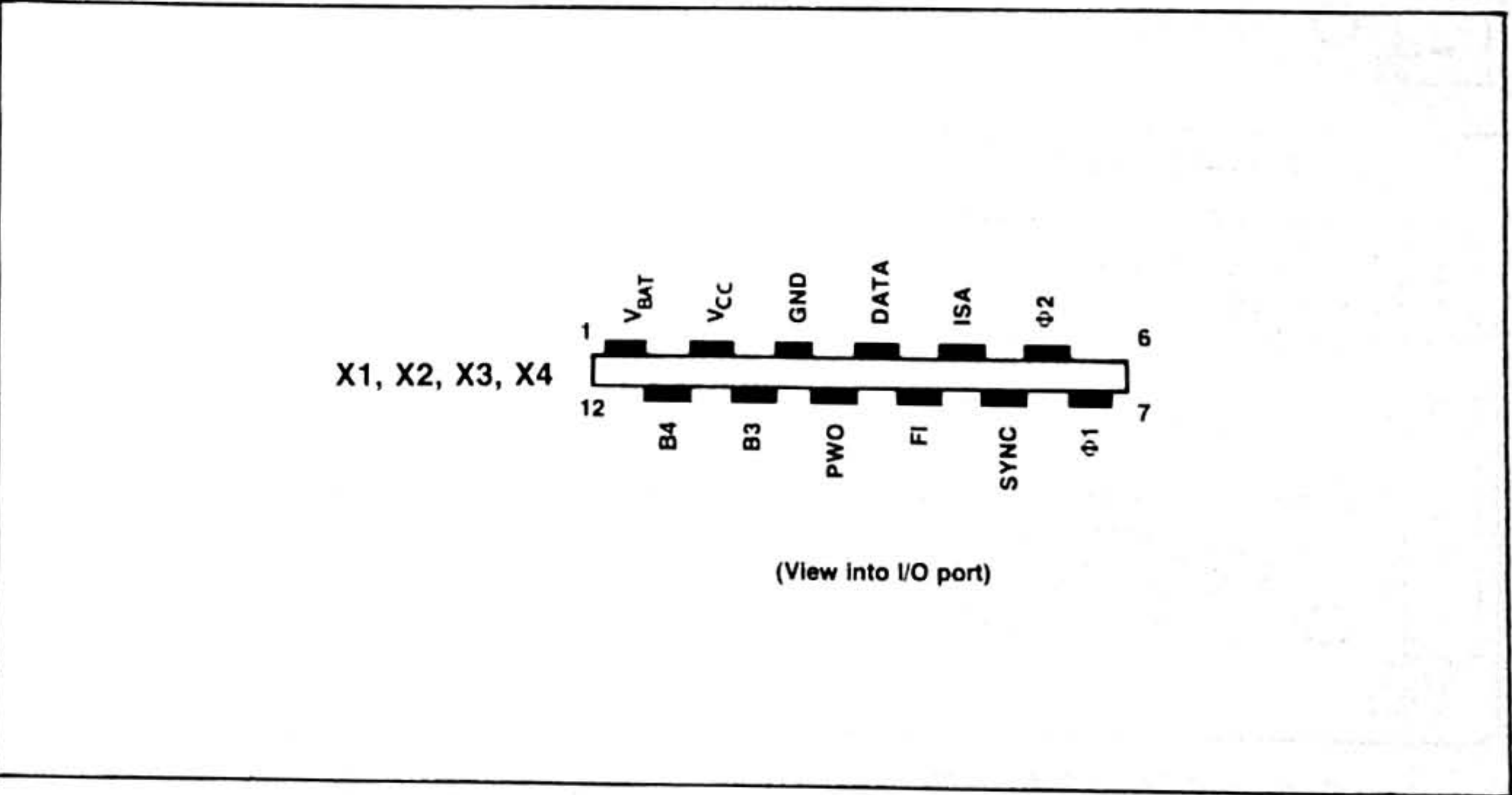
Figure 4-6. Contacts at I/O Port
