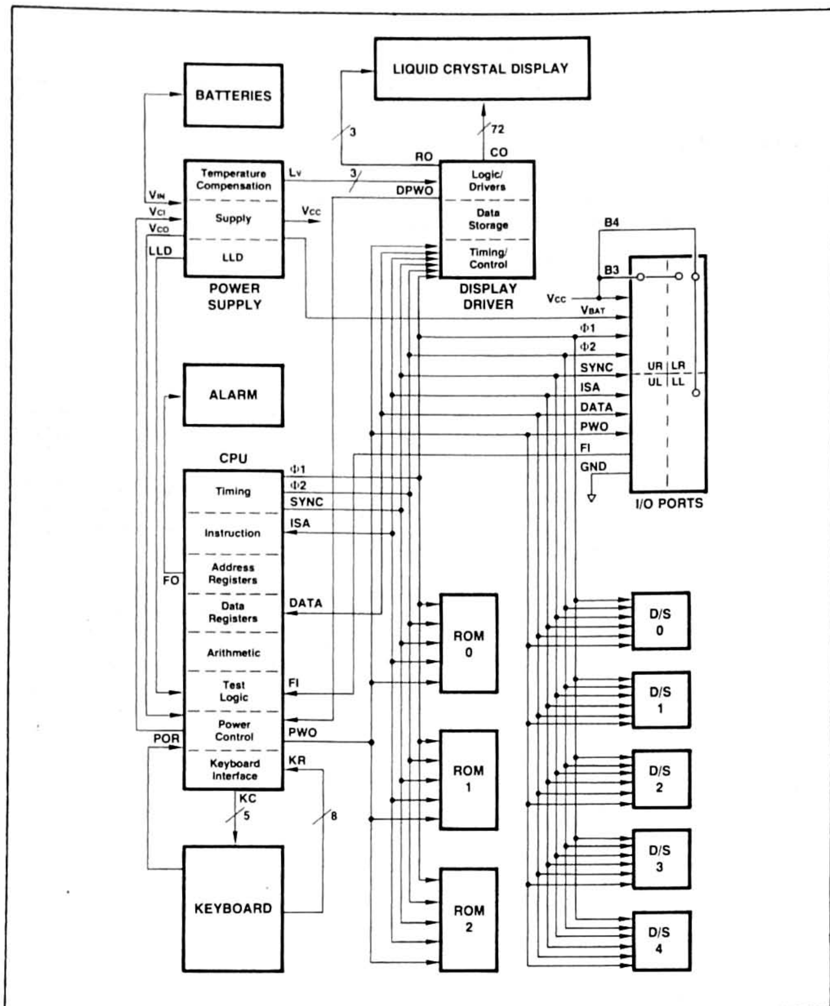
Figure 2-1. HP-41C/CV Block Diagram
