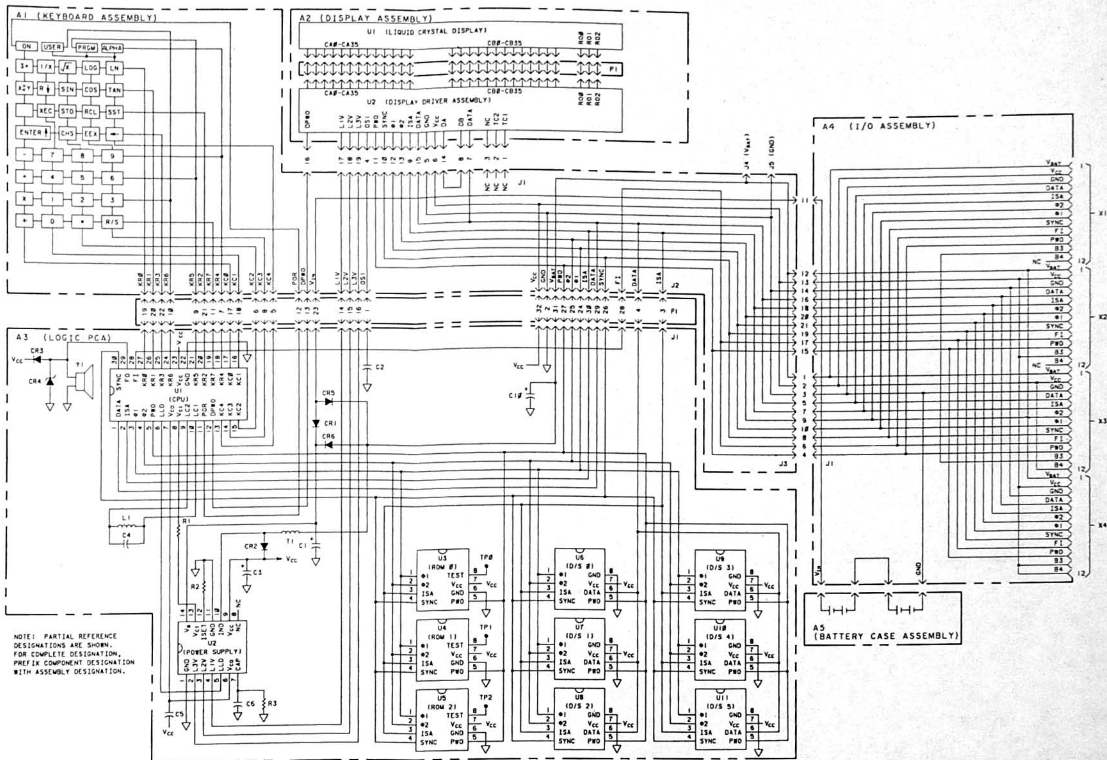
Figure 4-9d. Initial HP-41CV Schematic Diagram
