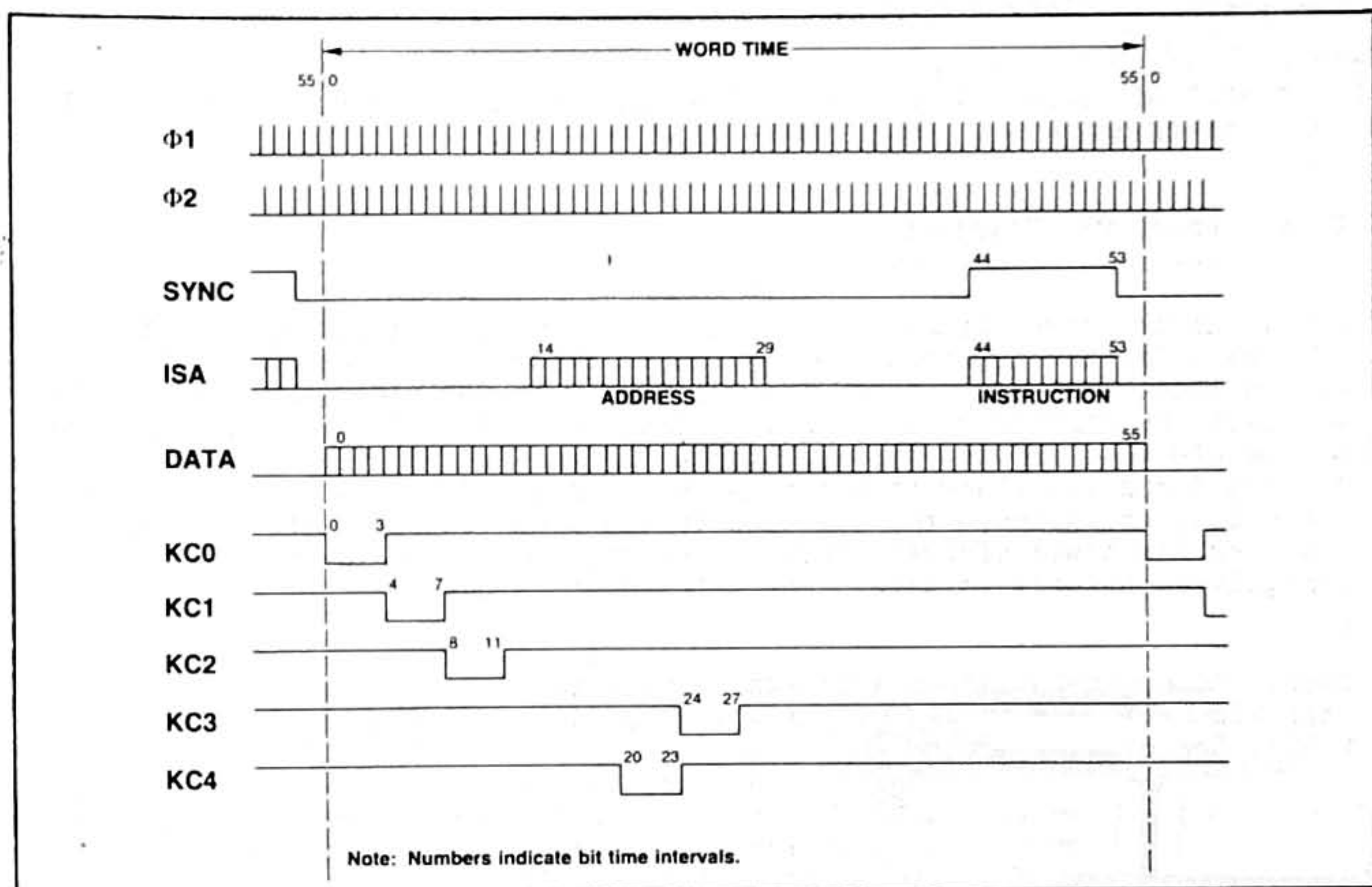
Figure 2-4. System Timing
