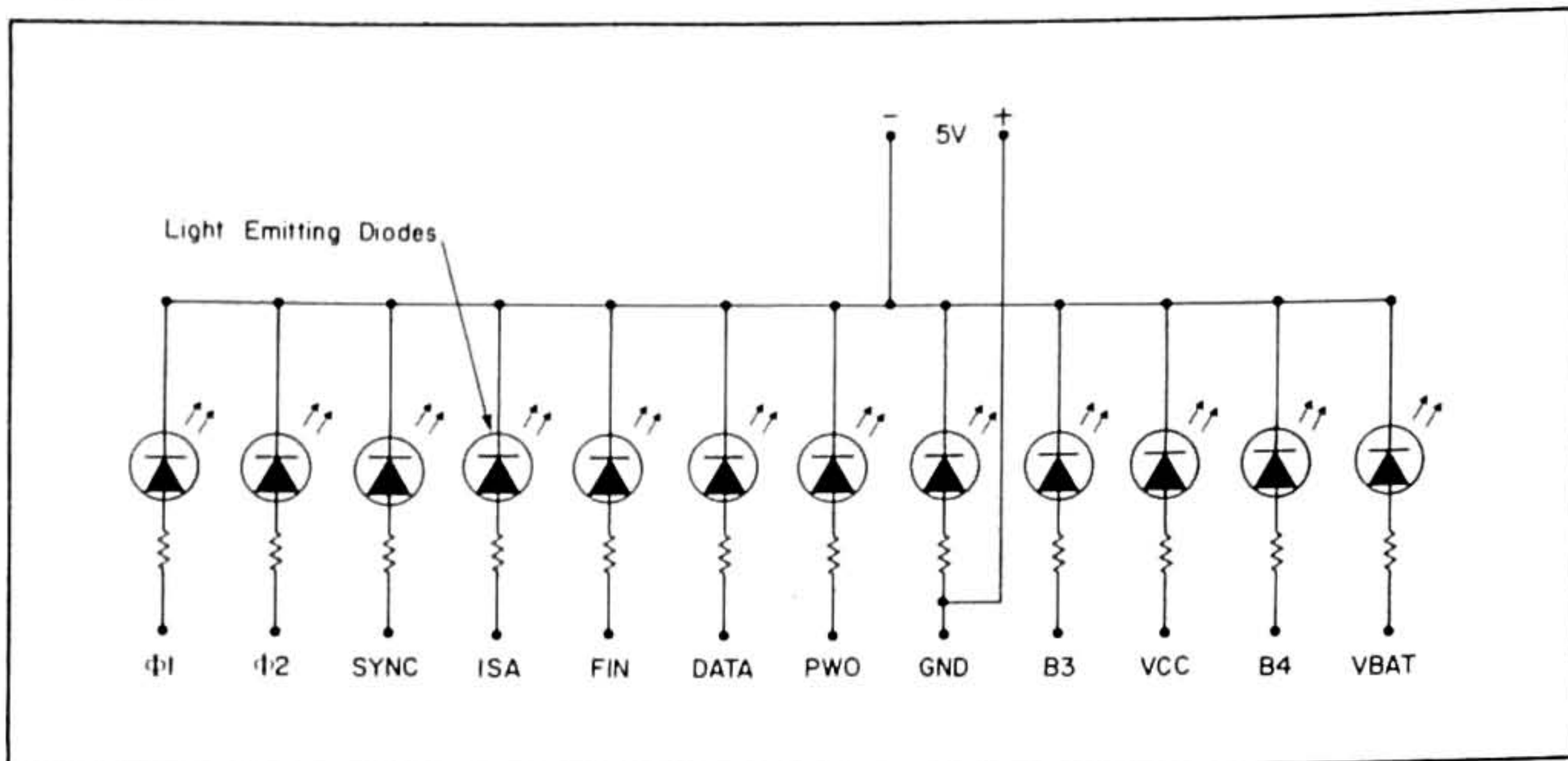
Figure 4-4. Port Extender Modification Schematic
