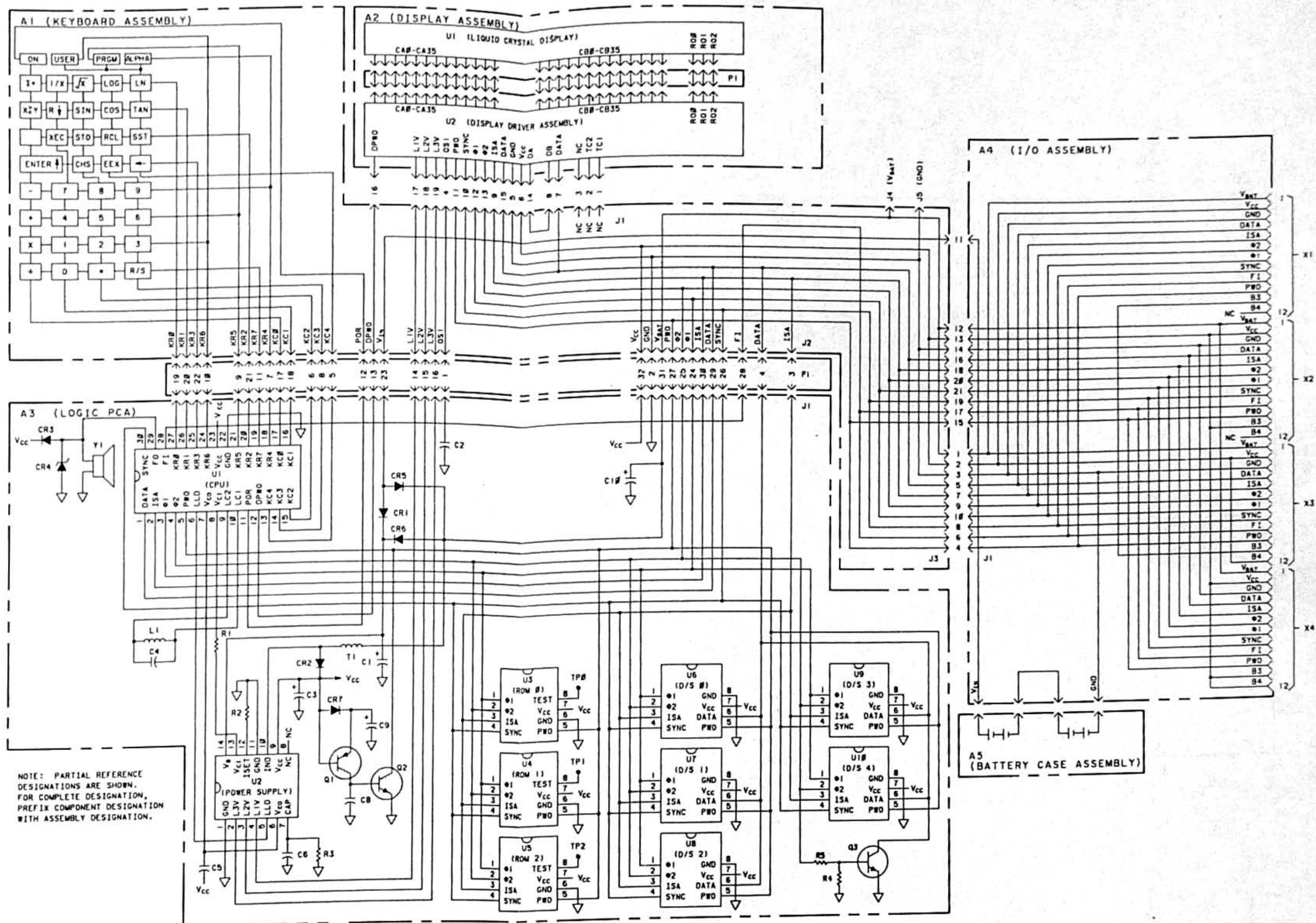
Figure 4-9a. Initial HP-41C Schematic Diagram
