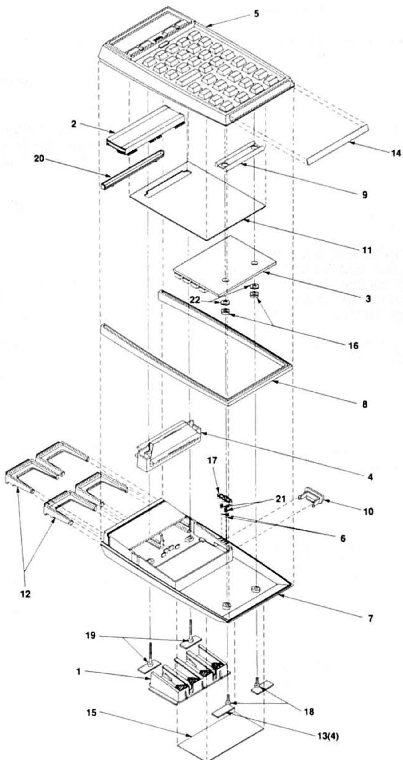
Figure 6-1. HP-41 Exploded View
