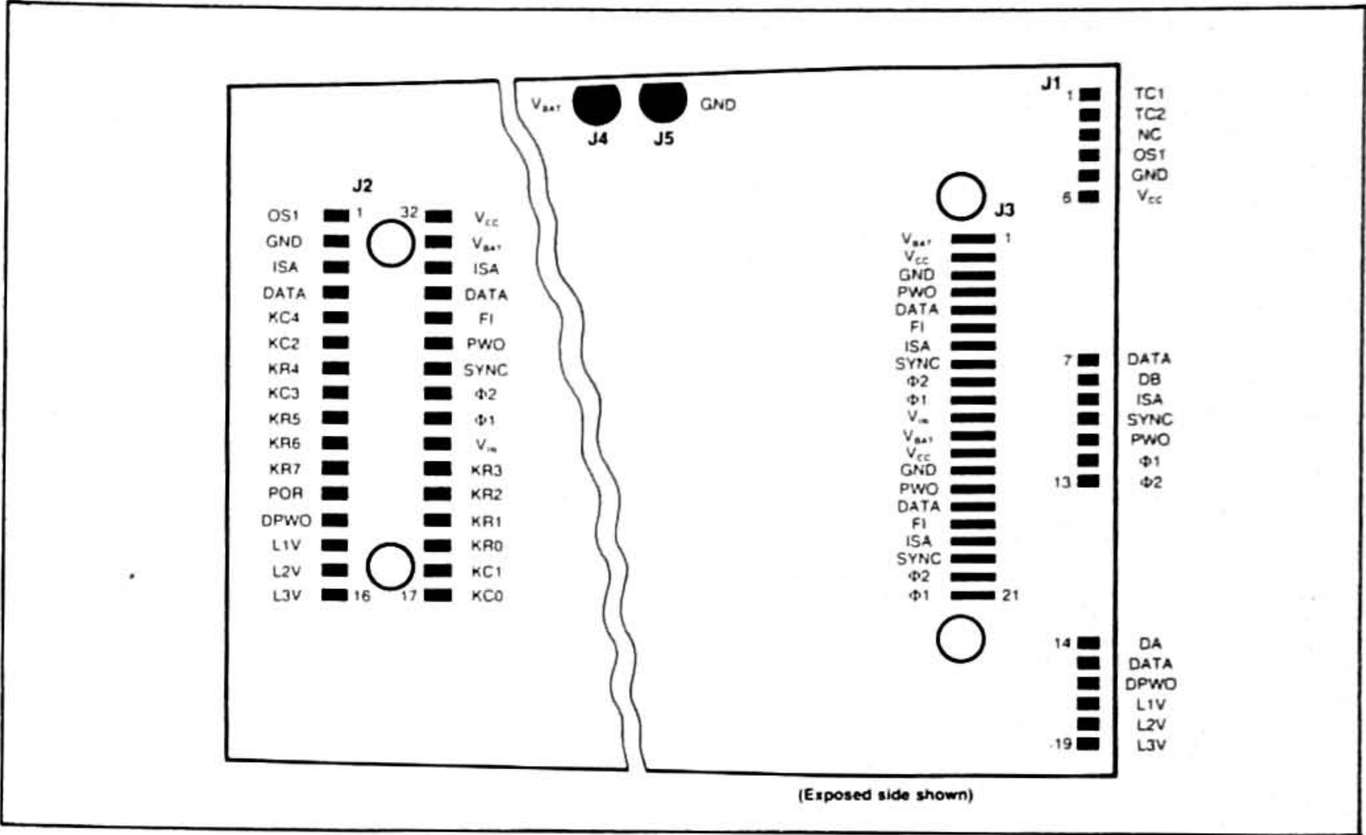
Figure 4-5. Contacts on Keyboard PC Board
