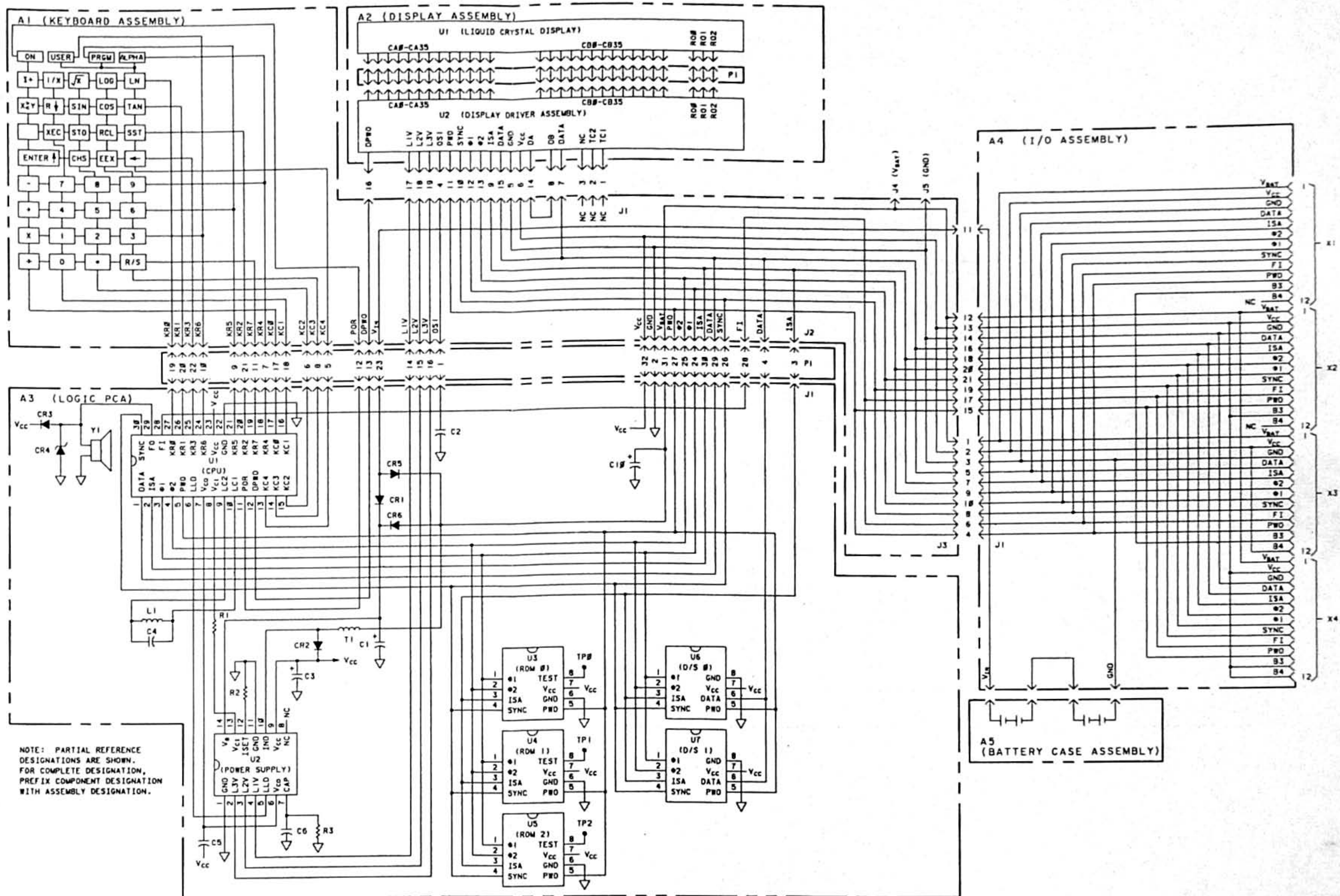
Figure 4-9c. Final HP-41C PCA Schematic Diagram
