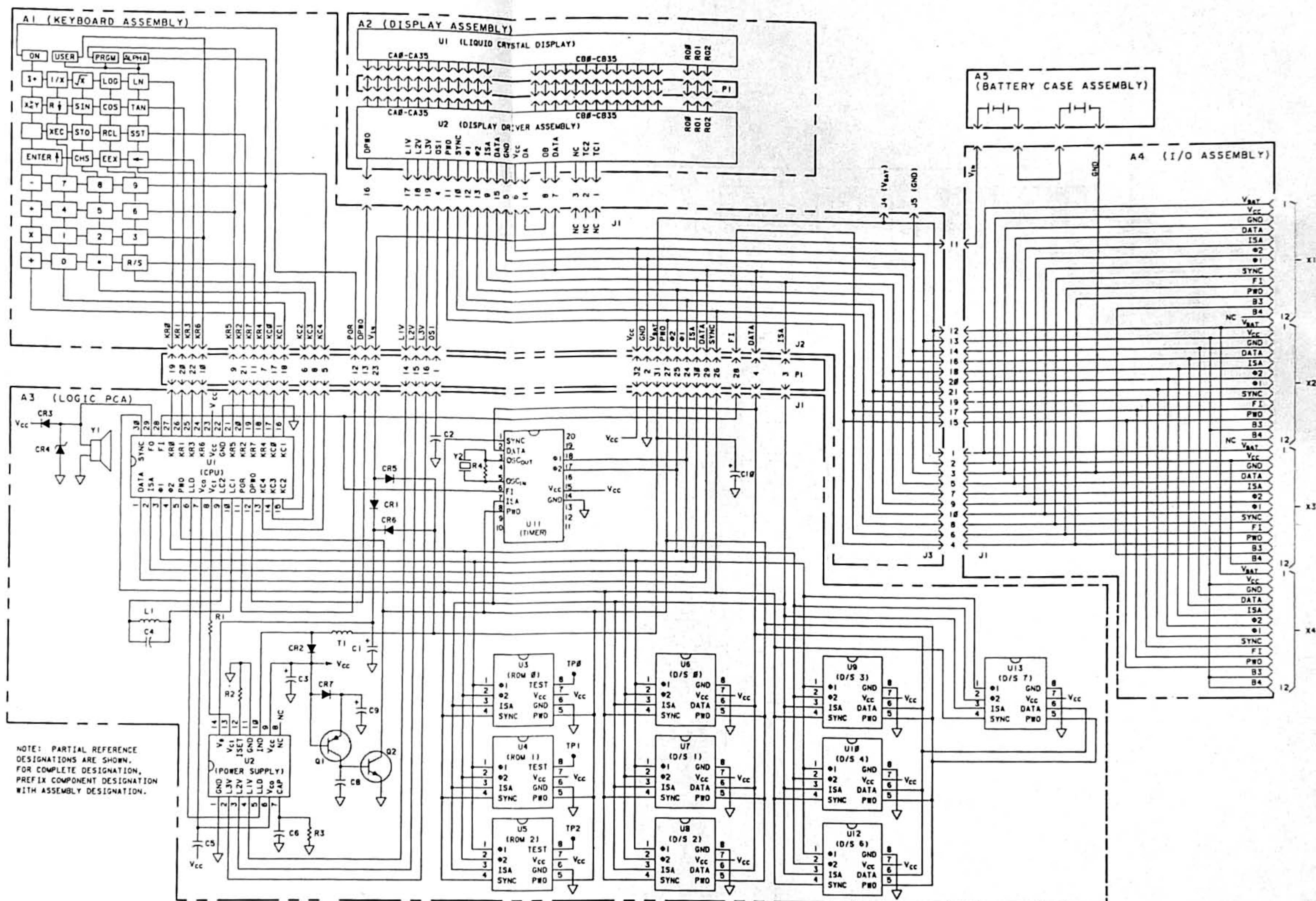
Figure 4-9f. HP-41C/CV/CX Common Board Schematic Diagram
