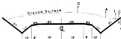
Road Cross Section Design Template
