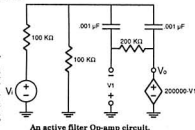
An active filter Op-amp circuit.
